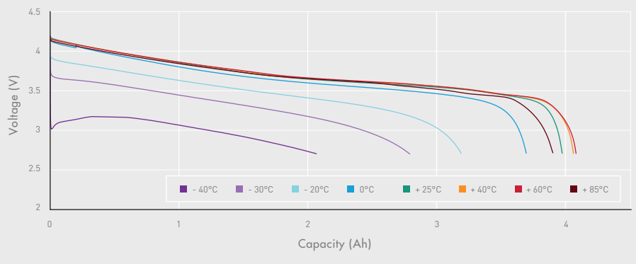
Typical discharge profiles (0.8 A - C/5 rate)
