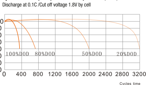
Cycle life curves (25°C) / Courbes de cycle de vie (25°C)
