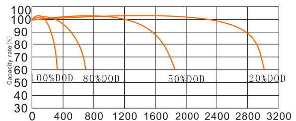
Cycle life curves (25°C) / Courbes de cycle de vie (25°C) Discharge at 0.1C / Cut off voltage 1.8V by cell
